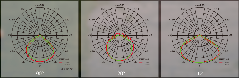
Light Distribution Curve
